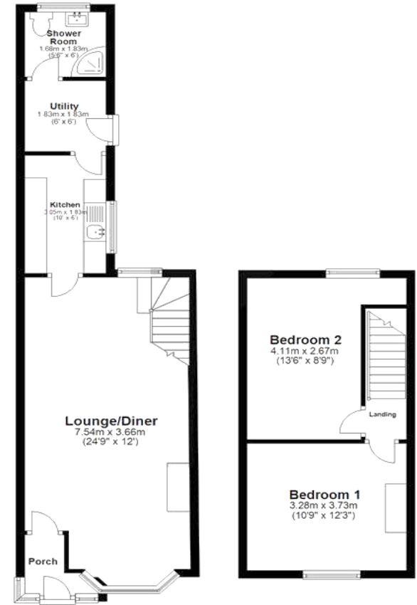
Floor Plan for illustrative purposes only
